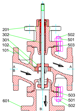
MV 5331, PV 6331 DN 20 – 80, PN 16 – 40
