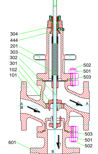
MV 5334, PV 6334 DN 20 – 150, PN 16 – 25
