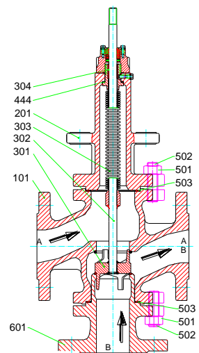
MV 5324, PV 6324 DN 20 – 150, PN 16 – 25
