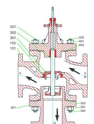
MV 5331, PV 6331 DN 65 – 150, PN 63 – 100
